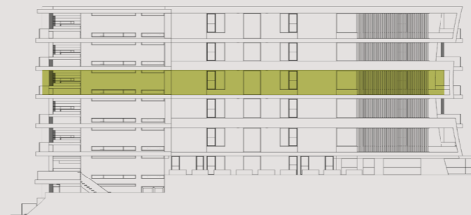
NORTHERN ELEVATION
